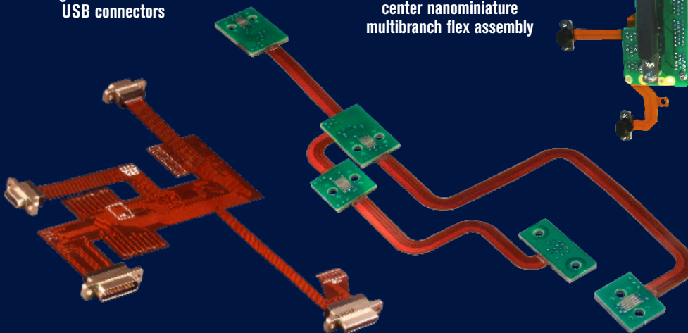
Hybrid flex/rigid multibranch assembly ready for connector termination
