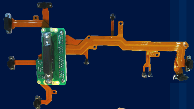
Multibranch factory demo rigid flex assembly highlighting the broad range of catalog board and mezzanine connectors available from Glenair
